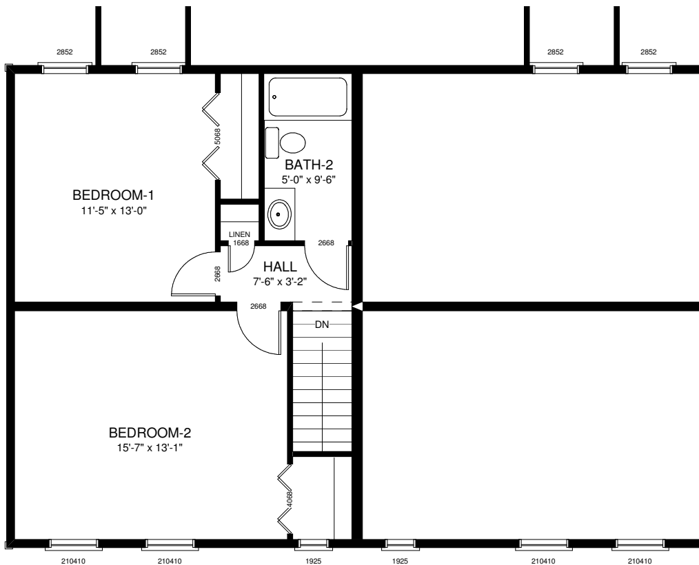
PLAN SECOND FLOOR
