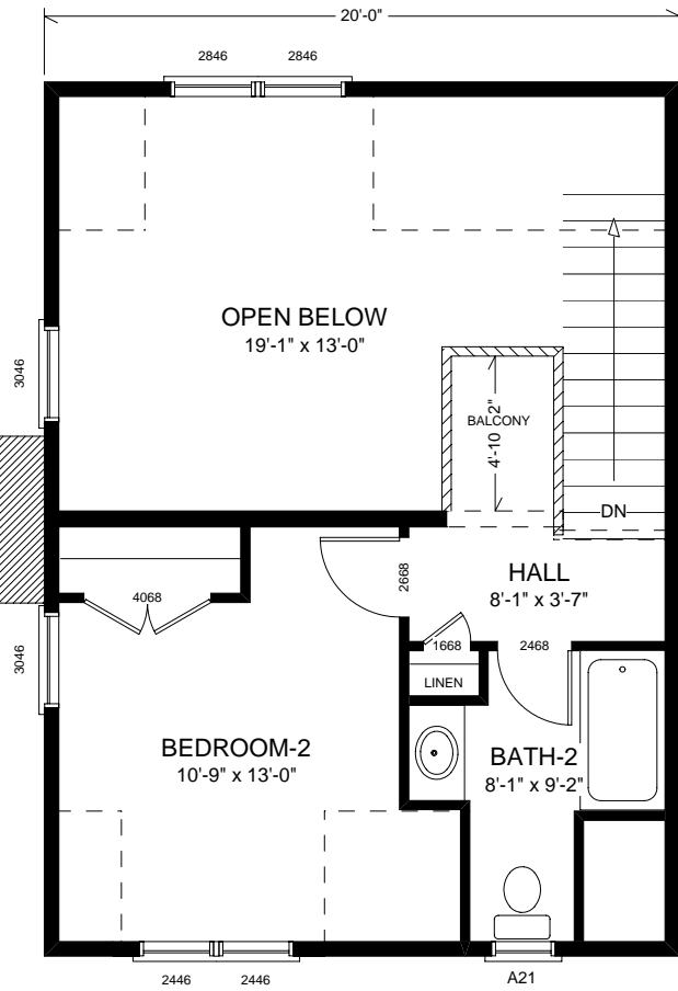
UNIT "A" PLAN SECOND FLOOR
